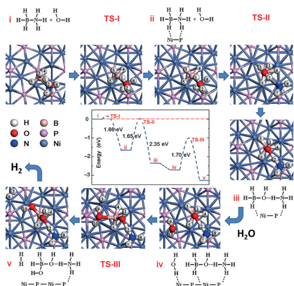
Figure 4. Plot of energy changes versus reaction coordinate calculated for \text{Ni}_2\text{P} -catalyzed hydrolysis of AB.
