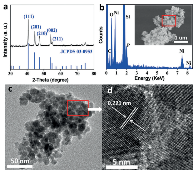
Figure 1. a) XRD pattern and b) EDX results corresponding to a selected scanning electron microscope image (inset); c) TEM and d) HRTEM images of obtained Ni 2 P NPs.
