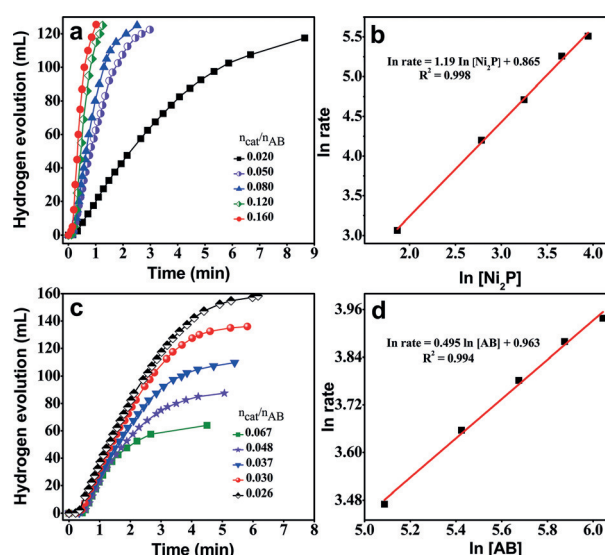
Figure 2. a) Stoichiometric hydrogen evolution in aqueous solution (5 mL) containing fixed amount of AB (1.62 mmol) at various Ni 2 P/AB molar ratios at 298 K; c) relationship between hydrogen-generating rate and AB concentration at fixed amount (0.054 mmol) of Ni 2 P in water at 298 K; b), d) Logarithmic plots of rate versus [Ni 2 P] and [AB], respectively.
